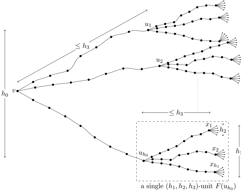
FIGURE 3. An (h_0, h_1, h_2, h_3) -web W .
